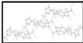
Fig. 2. The partial packing of (I), which shows that molecules form dimers which are inter-linked.
